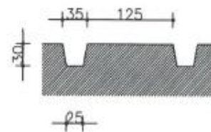
sleufdetail
